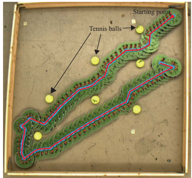
Fig. 8: The experimental results: the robot successfully avoids collisions with obstacles. The blue marker on top of the robot is used by the off-line tracker to estimate the robot's position and orientation.
