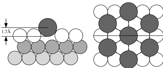
FIG. 16. Structural model showing the adsorption geometry for Na atoms substituting Al atoms on the Al(111) surface, see Ref. 14. Open and light gray circles represent Al atoms in the first and subsequent layers, respectively; larger gray circles correspond to Na atoms.
