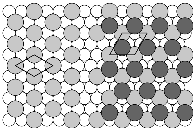
FIG. 14. Proposed model for the (2 \times 2) structure with two Na atoms per unit cell: one Na atom is on a substitutional adsorption site (gray), the second one is adsorbed (black). For comparison, the (\sqrt{3} \times \sqrt{3})R 30^\circ structure is shown on the left-hand side.
