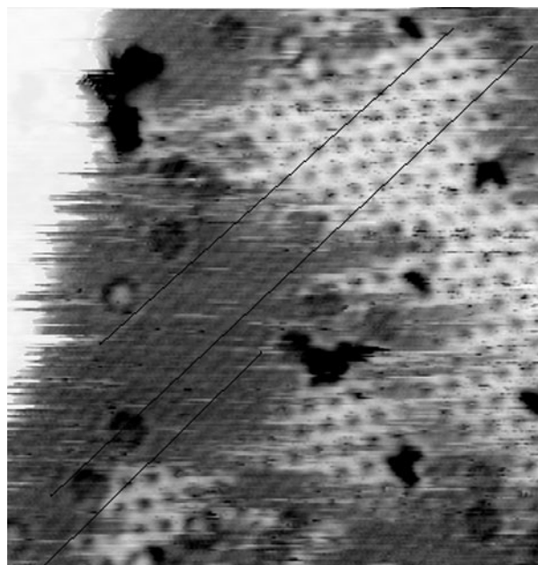
FIG. 5. Scanning-tunneling-microscopy topograph illustrating that Na atoms in the \sqrt{3} islands, imaged as depletions, are located in phase with the Au(111) surface atoms ( \Theta=0.15 , I_t=32 \text{ nA} , V_t=-0.5 \text{ V} , 103 \times 113 \text{ \AA}^2 ).
