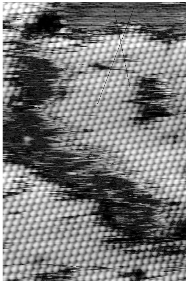
FIG. 3. Scanning-tunneling-microscopy image showing the atomic structure of the (\sqrt{3} \times \sqrt{3})R30^\circ phase formed by Na on Al(111) at T=300 K. Hexagonal arranged protrusions are identified as Na atoms. Dark areas represent clean substrate ( \Theta=0.24 , I_t=10 nA, V_t=-1.0 V, 123 \times 177 Å 2 ).
