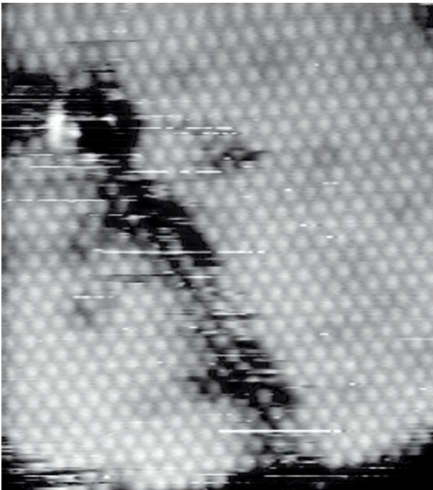
FIG. 7. Scanning-tunneling-microscopy topograph of two \sqrt{3} islands which are separated by a “light wall.” The streaks are due to fast exchange of atoms between the two islands ( \Theta=0.30 , I_t=3.0 nA, V_t=-1.2 V, 110\times 124 Å 2 ).
