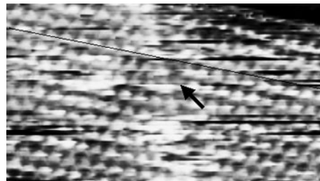
FIG. 8. Scanning-tunneling-microscopy images of the surface covered with a complete (\sqrt{3}\times\sqrt{3})R30^\circ Na monolayer, (a) overview, (b) and (c) details recorded at the rectangles marked in (a) which resolve the atomic structure of the terraces. The surface shows step alignment; furthermore, domain boundaries change into “heavy” walls, imaged as bright stripes in (a) [ \Theta=0.33 , sharp (\sqrt{3}\times\sqrt{3})R30^\circ LEED pattern, (a) I_t=3.0 nA, V_t=-1.2 V, 870\times 870 Å; (b) I_t=3.0 nA, V_t=-0.5 V, 260\times 240 Å 2 ; (c) detail from (b) 90\times 55 Å 2 ].
