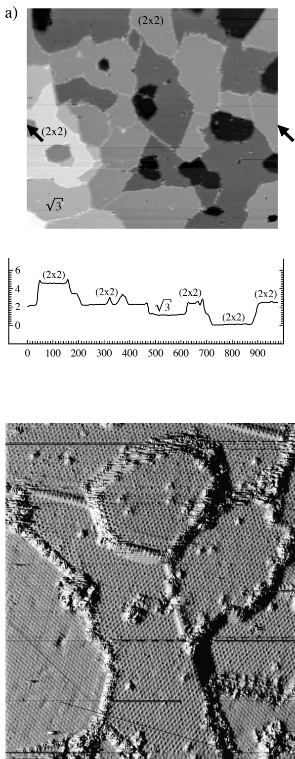
FIG. 12. Scanning-tunneling-microscopy images recorded on a surface with (2 \times 2) and \sqrt{3} phase coexistent. (a) Overview image, (b) higher resolution image of the area marked by a rectangle in (a), resolving the atomic structure of both phases. The overlap with the overview in (a) allows us to assign the structure to the areas imaged as different height levels, the line scan in (a) shows the identification of (2 \times 2) and \sqrt{3} areas by their imaging height [ \Theta = 0.40 , LEED (\sqrt{3} \times \sqrt{3})R 30^\circ coexistent with (2 \times 2) , (a) I_t = 13 nA, V_t = -1.0 V, 980 \times 900 \text{ \AA}^2 ; (b) I_t = 34 nA, V_t = -0.7 V, 362 \times 422 \text{ \AA}^2 ].
