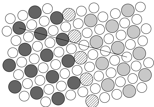
FIG. 9. Structural model (top view) of the two \sqrt{3} domains imaged in Fig. 8(c). Na atoms are sketched as filled circles, Al atoms with their smaller radius as smaller open circles, Na atoms introduced between the domains are represented as hatched circles, they presumably fluctuate between sites located on nearest-neighbor positions to the left and right domain.
