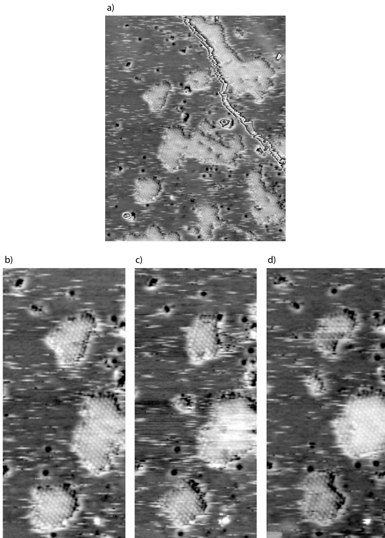
FIG. 6. Scanning-tunneling-microscopy images showing the evolution of the same area of the partly covered Al(111) surface with time. Images (b), (c), and (d) have been sequentially recorded each 125 s, (a) shows an overview. The mobility of Na is obvious from white stripes between the islands, representing a Na atom temporarily located under the tip, and from fluctuations of island sizes and shapes with time [ \Theta=0.12 , I_t=0.1 nA, V_t=-2.0 V; (a) 364 \times 460 \text{ \AA}^2 ; (b)–(d) 140 \times 308 \text{ \AA}^2 ].
