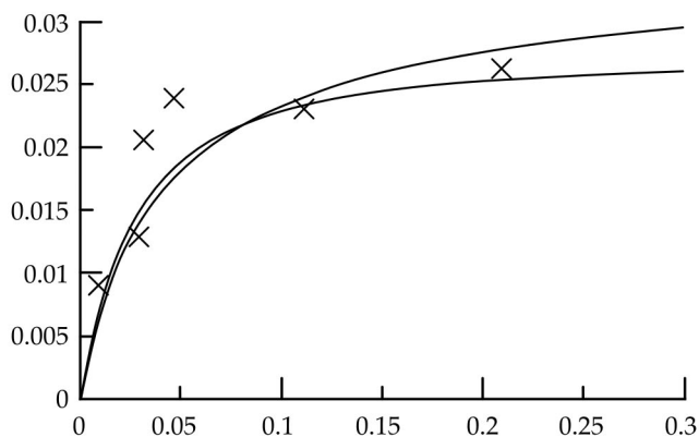
FIG. 16. Fit of the island density vs coverage derived from a model for hot adatom trapping [lower curve: \sigma (single atom) = 2.86 Å, \lambda = 160 Å, upper curve: \sigma = 8.58 Å, \lambda = 70 Å] to the experimental data from Fig. 6 (marked as x).
