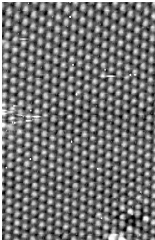
FIG. 2. STM image of clean Al(111) ( I_t=16 nA, U_t=-0.05 V, 46 Å \times 71 Å).
