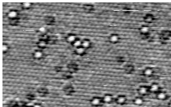
FIG. 3. Typical contaminations of the Al(111) surface after the sample has not been cleaned for several days. White features with dark rings represent carbon atoms ( I_t=9 nA, U_t=-0.36 V, 111 Å \times 69 Å).
