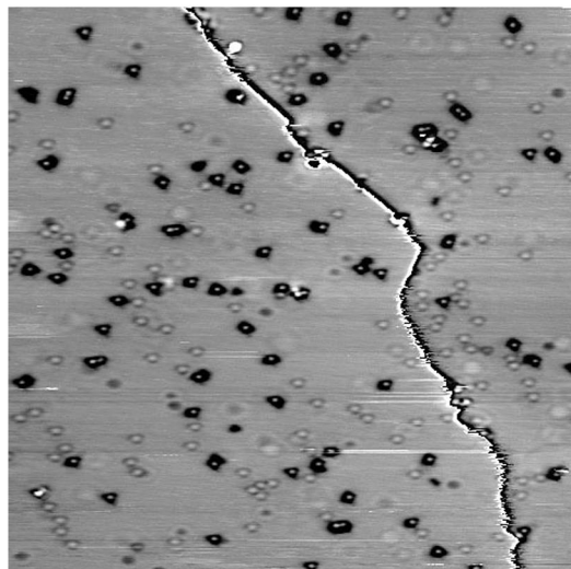
FIG. 7. STM image of Al(111) after 3 L \text{O}_2 exposure. Dark features with bright central spots are oxygen atoms ( I_t=8 nA, U_t=-0.5 V, 235 \text{ \AA} \times 227 \text{ \AA} ).
