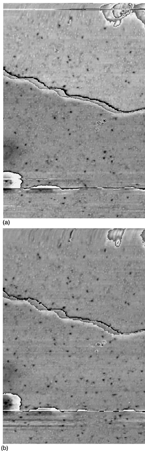
FIG. 8. STM topographs of three terraces of the Al(111) surface, showing individual oxygen adatoms (a) After 1.1 L O_2 , \Theta = 0.0014 \text{ ML} ; (b) after 2.1 L O_2 , \Theta = 0.0029 \text{ ML} ( I_t = 1 \text{ nA} , U_t = -0.2 \text{ V} , 474 \text{ \AA} \times 703 \text{ \AA} ).
