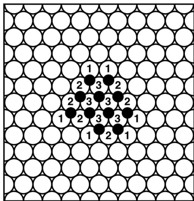
FIG. 17. Typical small ( 1 \times 1 ) O_{ad} island on Al(111). Indicated are the numbers of oxygen atoms (full dots) which are directly bound to aluminum atoms (open circles).
