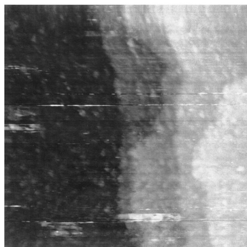
FIG. 13. Series of large scale images ( 660 \text{ \AA} \times 580 \text{ \AA} ) recorded on the same area during oxygen adsorption up to the oxidation range: (a) (almost) clean surface (2.4 L), (b) after 100 L, (c) 280 L, and (d) 790 L \text{O}_2 exposure ( p_{\text{O}_2} = 2 \times 10^{-8} Torr up to 1 \times 10^{-6} Torr, I_t = 0.1 \text{ nA} , U_t = -1 \text{ V} ).
