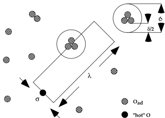
FIG. 18. Filled circle: hot oxygen adatom, shaded circles: thermalized oxygen atoms and islands. \sigma : cross section for a successful trapping event of the hot adatom at a thermalized island. \delta/2 : zone of influence around an oxygen atom or island. \lambda : ballistic path length of the hot adatom.
