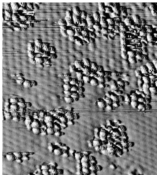
FIG. 11. Al(111) surface after 72 L O_2 exposure with (1 \times 1) oxygen islands. ( I_t=70 nA, U_t=-0.1 V, 66 Å \times 73 Å).
