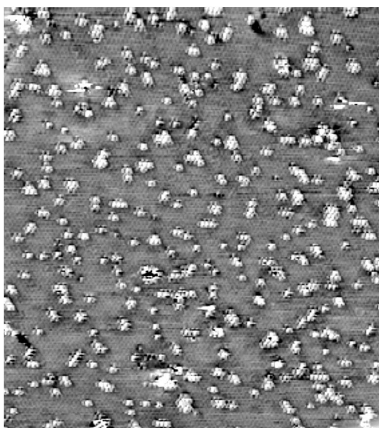
FIG. 10. Al(111) surface after 20 L O_2 exposure, showing small (1 \times 1) O_{ad} islands. ( I_t=11 nA, U_t=-0.1 V, 242 Å \times 271 Å).
