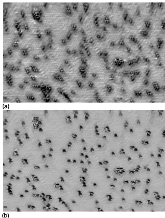
FIG. 5. STM images of the same surface area recorded with different tunnel currents corresponding to gap widths that differ by 0.5 \text{ \AA} : (a) I_t = 28 nA, (b) I_t = 70 nA, (exposure: 20 L \text{O}_2 , U_t = -0.1 V, 260 \text{ \AA} \times 92 \text{ \AA} ).
