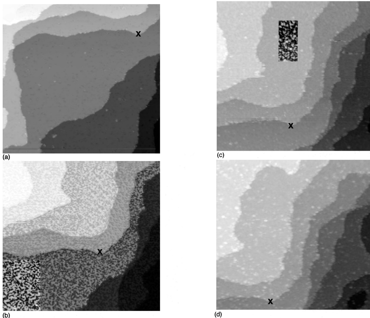
FIG. 13. Series of large scale images ( 660 \text{ \AA} \times 580 \text{ \AA} ) recorded on the same area during oxygen adsorption up to the oxidation range: (a) (almost) clean surface (2.4 L), (b) after 100 L, (c) 280 L, and (d) 790 L \text{O}_2 exposure ( p_{\text{O}_2} = 2 \times 10^{-8} Torr up to 1 \times 10^{-6} Torr, I_t = 0.1 \text{ nA} , U_t = -1 \text{ V} ).
