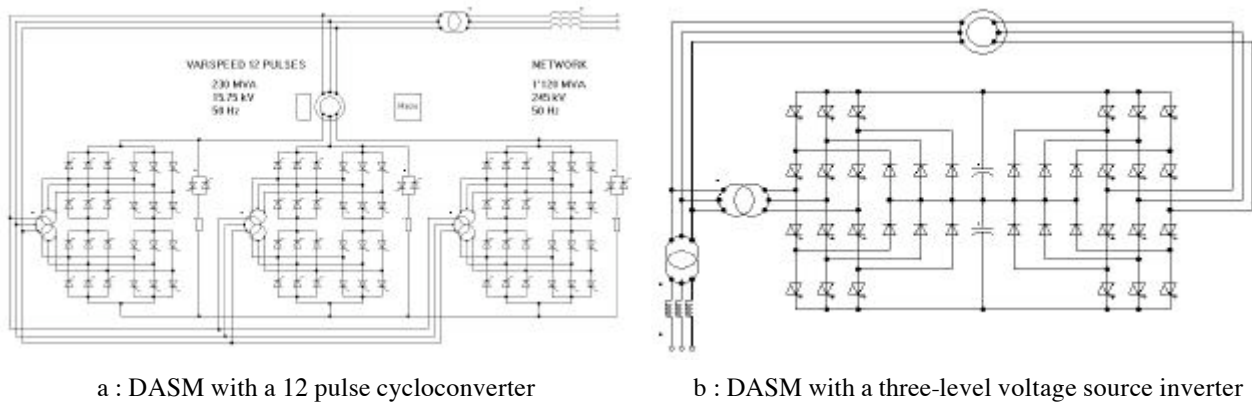
Figure 1 : DASM pumped storage groups
