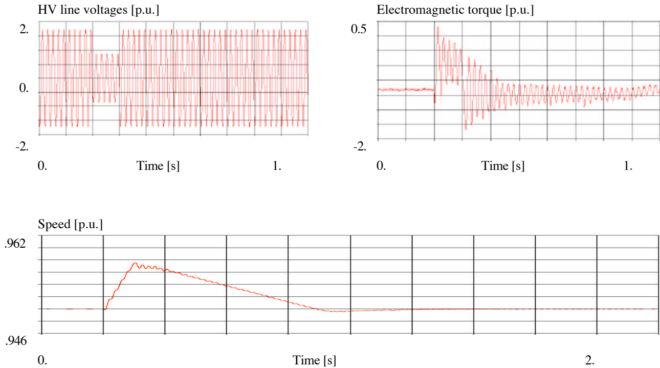
Figure 6 : voltage dip
