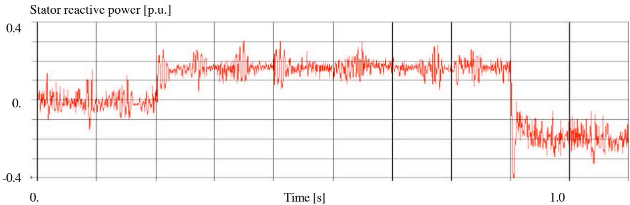
Figure 4 : reactive power control
