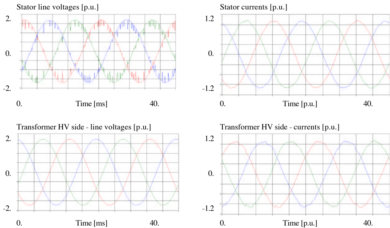
Figure 3 : steady state operation
