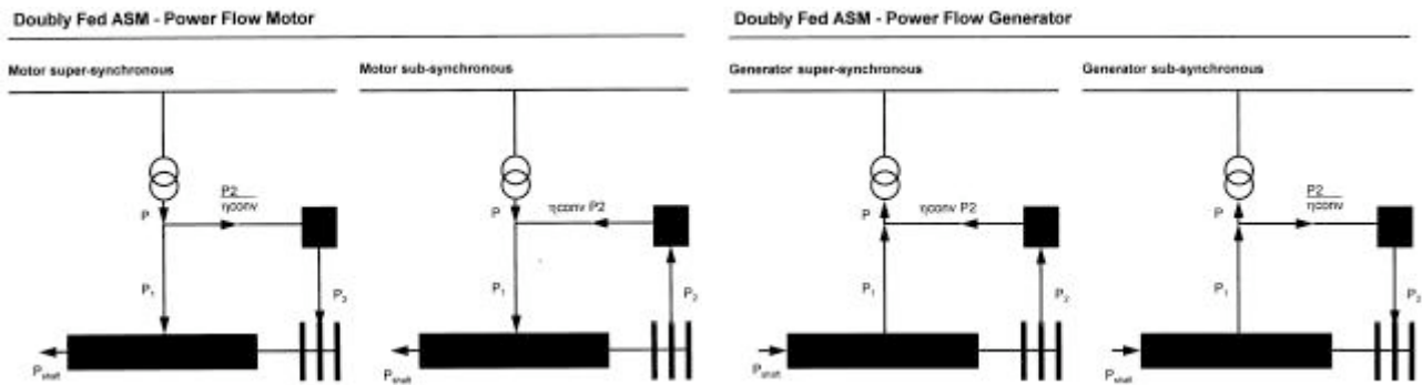
Figure 2 : power flows
