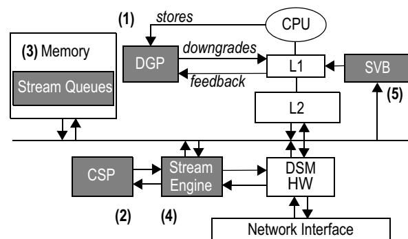
Figure 5. Anatomy of a SORDS-based DSM node.
