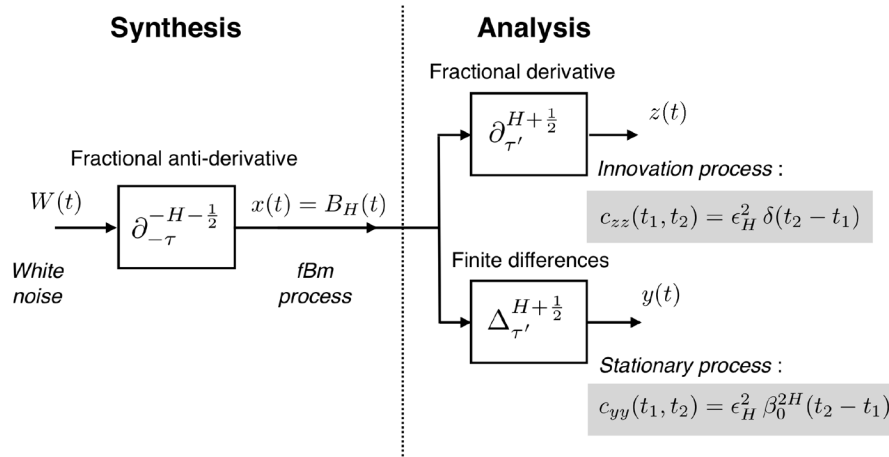
Fig. 1. Synthesis and analysis of a self-similar stochastic process: The fBm process x(t) is generated by fractional integration of white Gaussian noise with suitable initial condition that guarantee that E\{x(0)^2\} = 0 . The whitening operator of the process is a fractional derivative operator \partial_{\tau'}^\gamma , of corresponding order. Even though x(t) is not necessarily stationary, it can be transformed into a stationary process y(t) through the application of the fractional finite difference operator \Delta_{\tau'}^\gamma . Since \Delta_{\tau'}^\gamma is a “good” discrete approximation of the continuous-time operator \partial_{\tau'}^\gamma , the correlation function c_{yy}(\tau) is well defined and concentrated around the origin. In fact, this function may be thought of as a regularized version of the Dirac impulse. Note that \tau' can be chosen arbitrarily.
