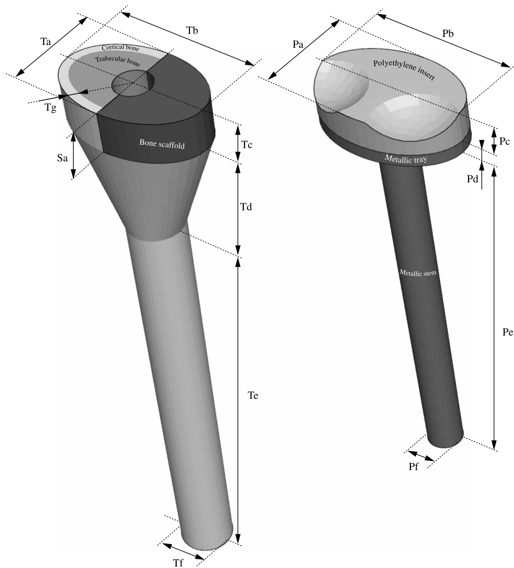
Figure 1. The revised tibia was modeled by a simplified geometry of the tibia, the artificial bone scaffold (left), and the revision knee prosthesis (right). The dimension values are given in Table 1.
