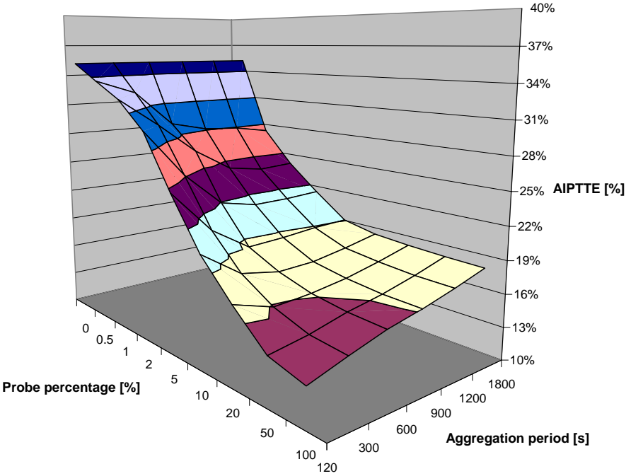
Figure 6: AIPSTE according to the aggregation period and the probe percentage for classical link definition
