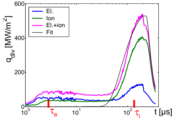
Figure 1. Power loads to the divertor plate during a Type-I ELM with W_{ELM} = 0.4 MJ.
