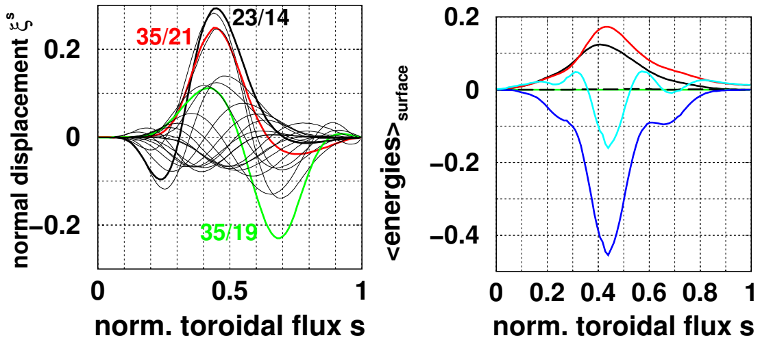
FIGURE 6. CAS3D normal displacement harmonics (left) and surface-averaged energy contributions (right) at \langle\beta\rangle = 0.22 . Radial integration of the surface-averages of \delta^2W (curve oscillating around zero) shows it to be slightly positive.
