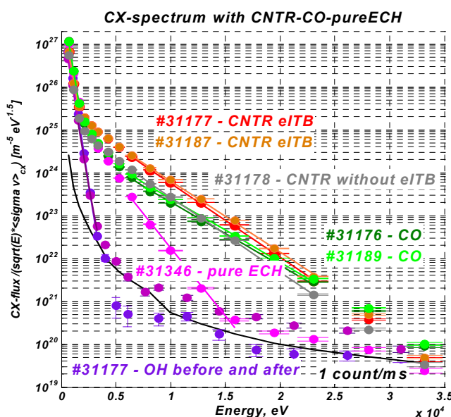
Fig.2: CNPA "CX-spectrums" in TCV plasma discharges with suprathermal ion populations.
