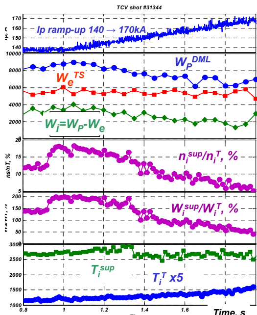
Fig.5: Plasma parameters in the TCV discharge with plasma current ramp-up.
