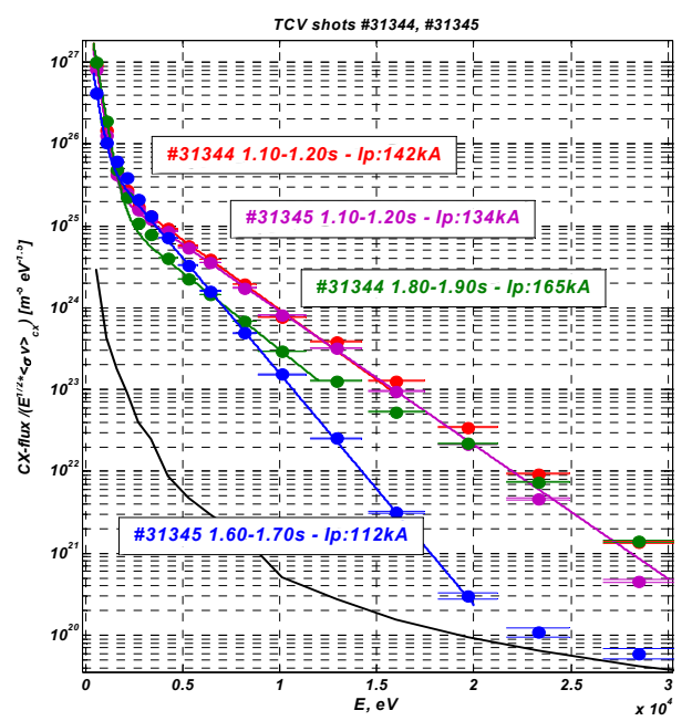
Fig.6: ‘‘CX-spectrums’’ for different plasma current.
