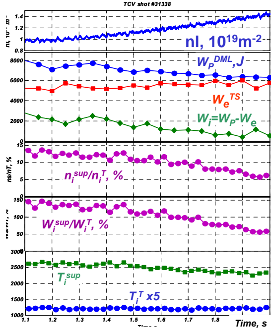
Fig.7: Plasma parameters in the TCV discharge with plasma density ramp-up.
