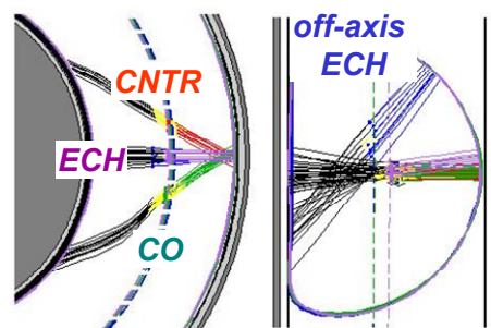
Fig.1: Gyrotrons alignment: ray-traces from TORAY calculation.
