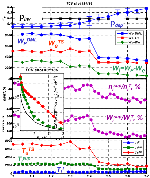
Fig.4: Parameters of the suprathermal ions in the TCV discharge with ramp-down the toroidal magnetic field. The decrease of magnetic field from 1.42 to 1.24 T leads to the shift of EC deposition from 0.03 to 0.40 in \rho_{\psi} .
