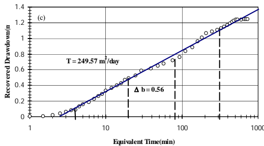
Figure 6. Deh-Pialeh piezometer (18 m deep) recovery data resulting from switching off the 50 m deep pumping well.
