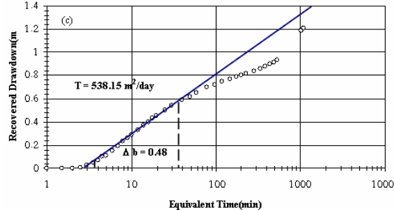
Figure 13. Dashte-Chenar piezometer (132m deep) recovery data.
