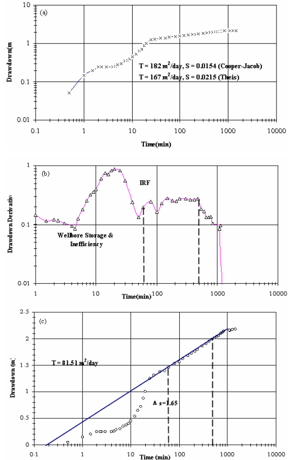
Figure 17. Katasbes piezometer (18m deep) drawdown data.
