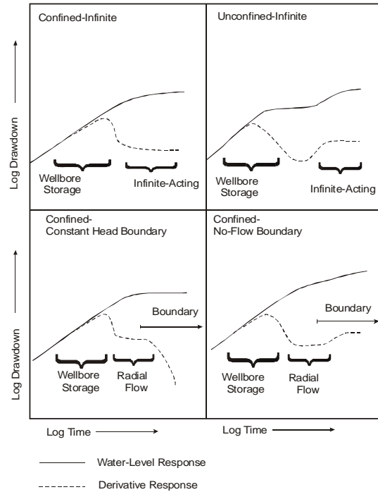
Figure 1. Characteristic log-log pressure and pressure derivative plots for various hydrogeologic formation/boundary conditions (after Spane and Wurstner, 1993).
