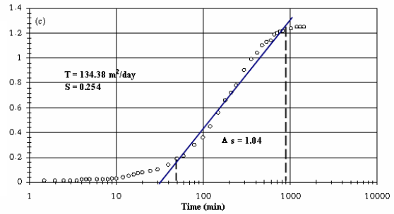
Figure 5. Deh-Pialeh piezometer (18 m deep) drawdown data.
