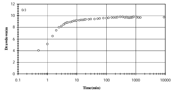
Figure 7. Dashte-Chenar pumping well (50 m deep) drawdown data.
