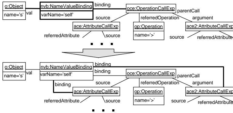
Fig. 8 Binding Passing
