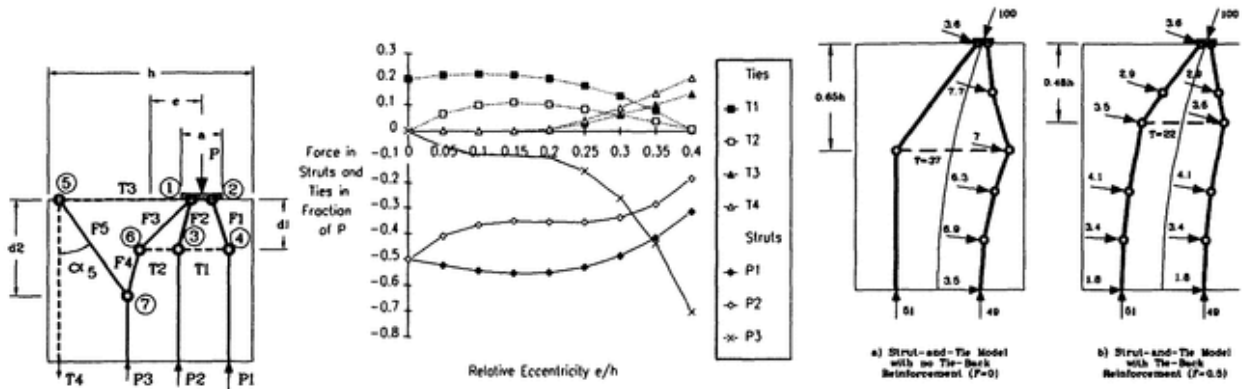
Figure 6: Strut-and-Tie Model of an Eccentric Function of the Anchorage Zone Figure 7: Forces in the Struts and Ties as a Function of the Eccentricity Figure 8: Strut-and-Tie Model of an Anchorage Zone with a Curved Tendon, Eccentricity 0.25h and Initial Inclination 20 degrees
