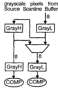
Figure 8 - The datapath followed by the grayscale pixels.
