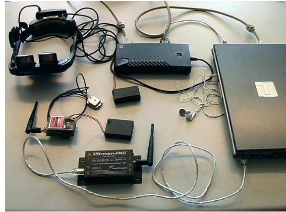
Figure 1: Required equipment for a typical wearable Augmented Reality framework: a notebook, a stereographic see-through HMD, a GPS antenna, some battery packs.
