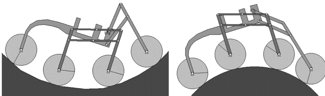
Figure 3 : Rover in a concave and convex ground
