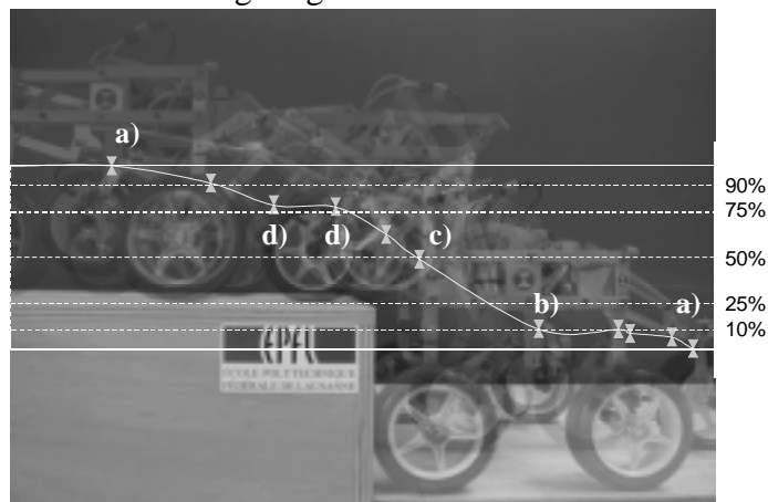
Figure 12 : Trajectory of the gravity center with the corresponding configurations defined in fig. 8
