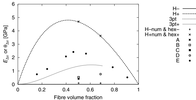
Fig. 11. Comparison of analytical bounds for soft elastic, nearly incompressible behaviour, with FEA solutions for elastic–plastic behaviour. The analytical solutions are taken from Fig. 6(b), the numerical ones from Fig. 6(c).
