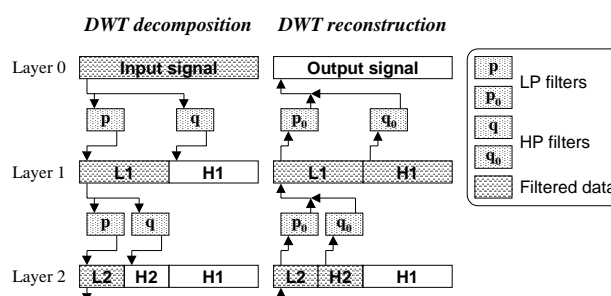
Figure 1: 1D DWT with Mallat tree decomposition. The number of samples of the encoded signal is equal to the one of the input signal.
