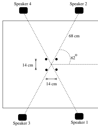
Figure 3: Experimental setup
