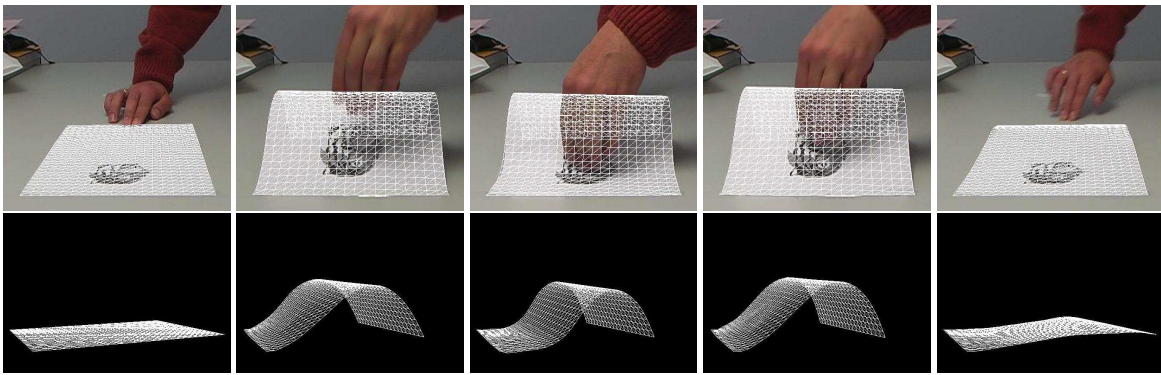
Figure 4: Occlusion handling. The front of the paper is taped to the table and one hand pushes the back of the page while the other passes in front. Top row: The recovered mesh is overlaid on the images. Note that the hand is in front of the paper even though the wireframed display gives the impression that it is behind. Bottom row: Side view of the recovered mesh. Note that its shape is undisturbed by the occlusion and that the back of the mesh also deforms correctly. A video of the sequence is given as supplementary material.
