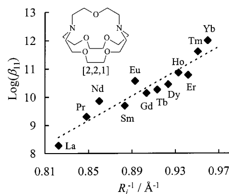
Figure 12. Formation constants of the cryptates [\text{Ln}[\text{2,2,1}]]^{3+} in methanol in functions of the inverse of nine-coordinate lanthanide ionic radii. 104 Units for \beta_{11} = \text{M}^{-1} .
