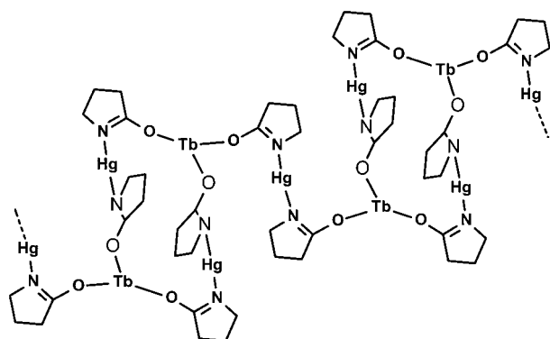
Figure 27. Schematic representation of the polymeric chain compound \{[\text{Hg}_3\text{Ln}_2\text{L}_6(\text{NO}_3)_6]\}_\infty (Ln = Gd). (Redrawn from ref 212.)
