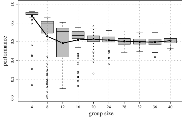
Figure 6: Scalability of the aggregation behavior. The performance for some group sizes (4, 8, 12, . . . , 40 s-bots ) is shown. The box-plot shows 100 evaluations per box. The average values are indicated by the thick black line. Boxes represent the inter-quartile range of the data, while the horizontal bars inside the boxes mark the median values. The whiskers extends to the most extreme data points within 1.5 of the inter-quartile range from the box. The empty circles mark the outliers.
