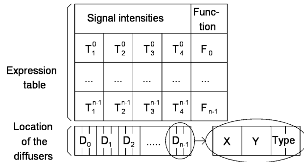
Fig. 3. The genetic code contains two parts. The first is the expression table T , here with n entries. Each entry is 16 bits long. The second part contains the location of the diffusers and their type. The number of bits for the X and Y coordinates depends on the size of the network. The type of the diffuser is encoded on 2 bits.
