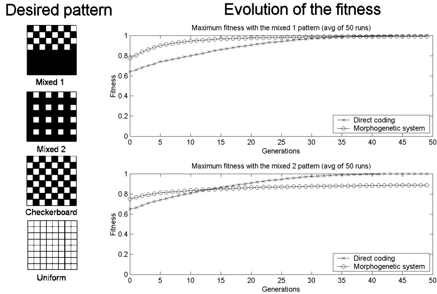
Fig. 4. The pattern coverage experiment consists in covering an array of 8x8 cells with a binary pattern. The left column shows the four desired pattern ( mixed1 , mixed2 , checkerboard and uniform ). The right column shows the evolution of the maximum fitness for the mixed1 and mixed2 patterns.
