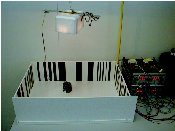
Figure 1: A Khepera robot equipped with a linear camera is positioned in an arena lit from above in order to let the evolutionary experiments continue at night. The robot is connected to a workstation through rotating contacts that provide serial data transmission and power supply. The spiking networks and genetic operators run on the workstation.
