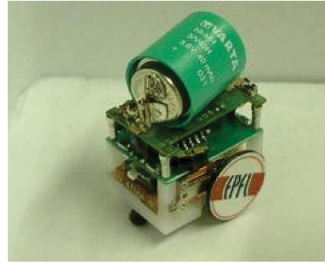
Figure 9: The mobile micro-robot Alice with the extra battery module providing up to 10 hour of energetic autonomy.
