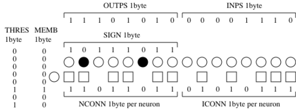
Figure 7: Digital representation of one neuron in the microcontroller.
