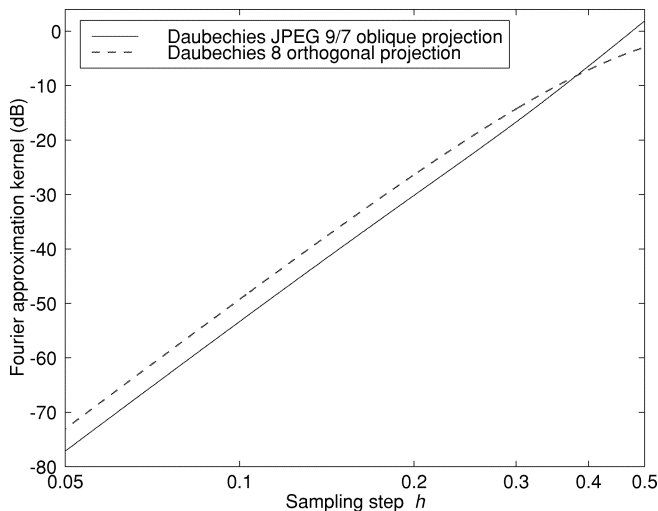
Fig. 6. Fourier approximation kernel corresponding to Daubechies JPEG 9/7, compared to Daubechies of same order.
