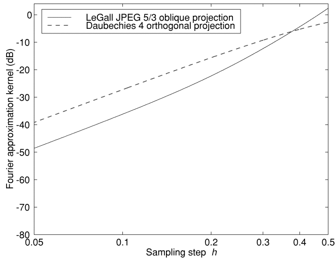
Fig. 3. Fourier approximation kernel corresponding to LeGall JPEG 5/3, compared to Daubechies of same order.
