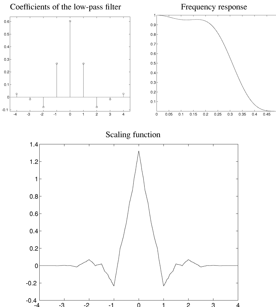
Fig. 4. Analysis Daubechies JPEG filter of length 9 and corresponding scaling function.
