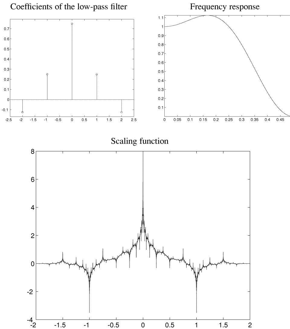
Fig. 1. Analysis LeGall JPEG filter of length 5 and corresponding scaling function.
