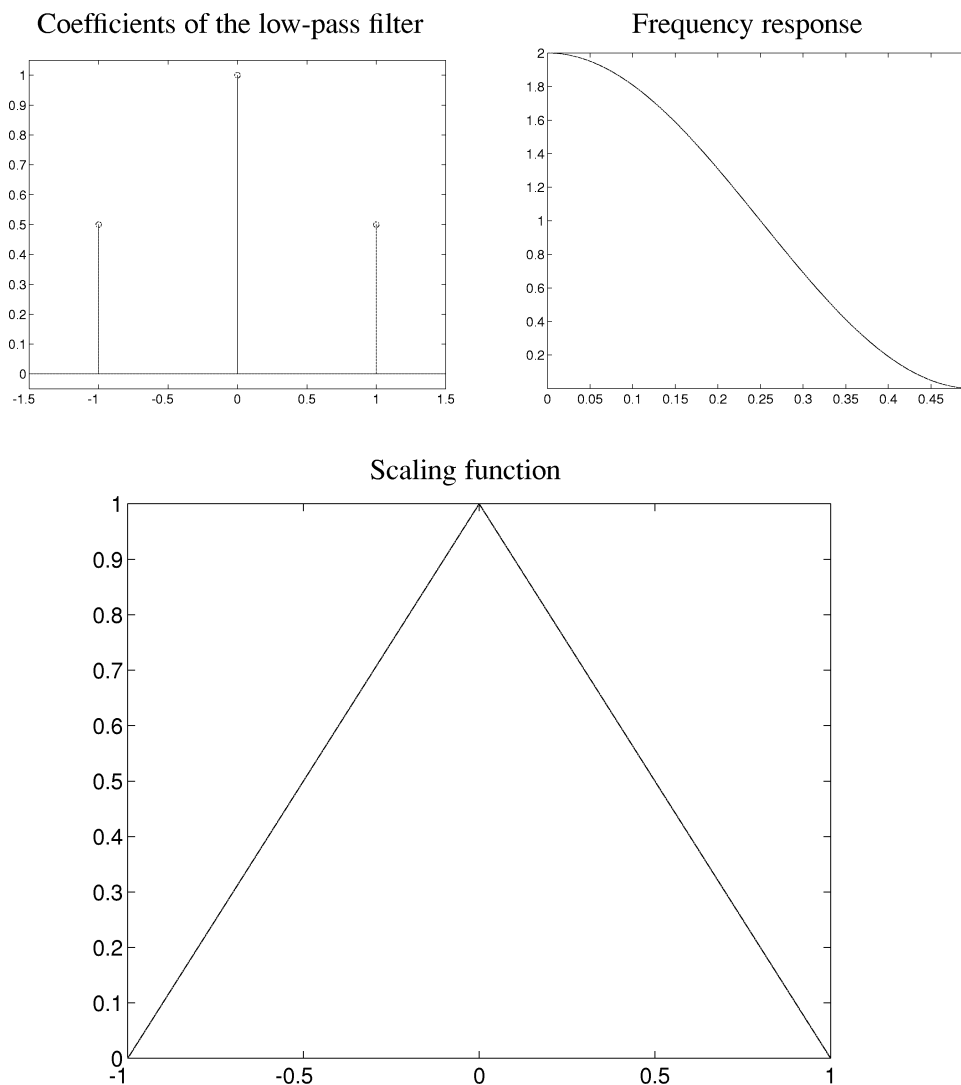
Fig. 2. Synthesis LeGall JPEG filter of length 3 and corresponding scaling function (i.e., \beta^1 , B-spline of degree 1).
