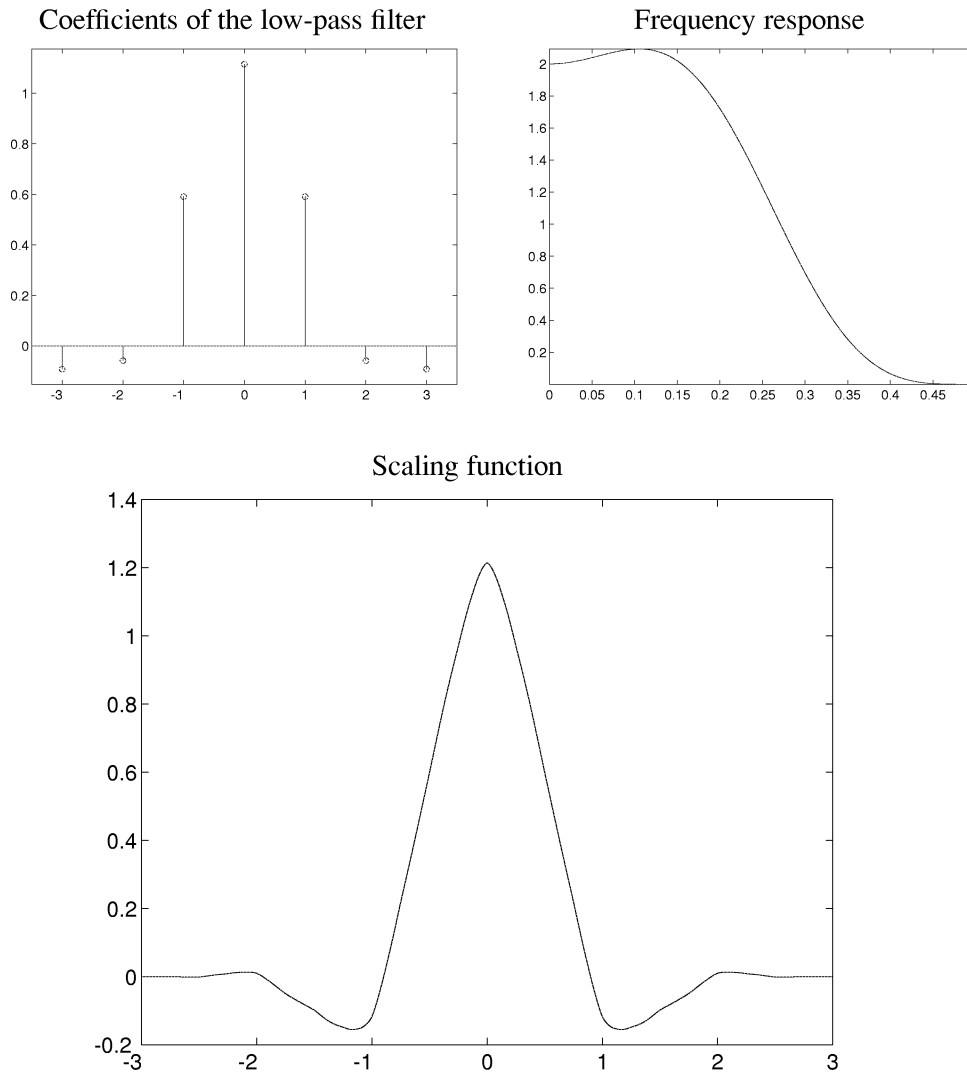
Fig. 5. Synthesis Daubechies JPEG filter of length 7 and corresponding scaling function.
