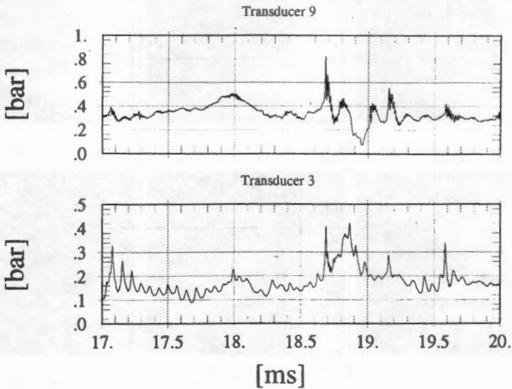
Figure 11: Pressure signals from transducers n°3 and n°9
