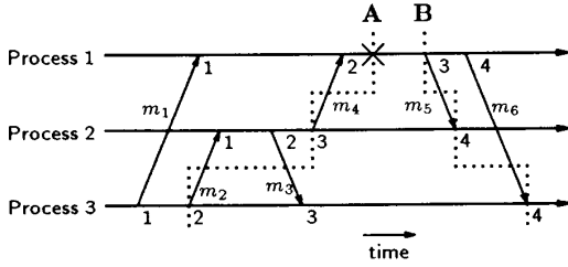
Figure 1 Distributed Breakpoints for Event 3 of Process 1.
