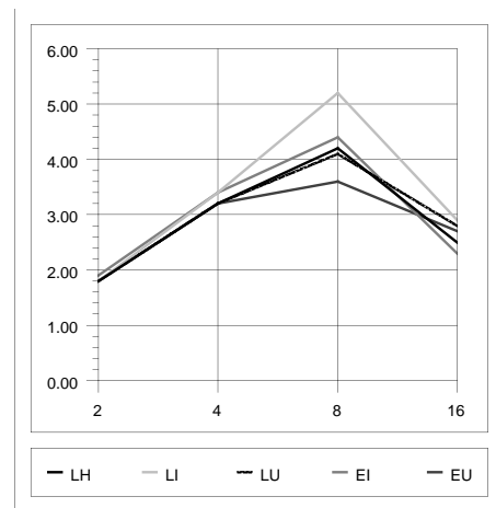
Figure 6 Speedup for Jacobi on Ethernet
