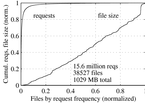
Figure 6: IBM Trace
