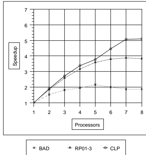
Figure 1: Speedup on an Ethernet Network - Different pedigrees
