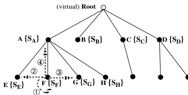
Fig. 4. Illustration of the GPCRDB thesaurus hierarchy
