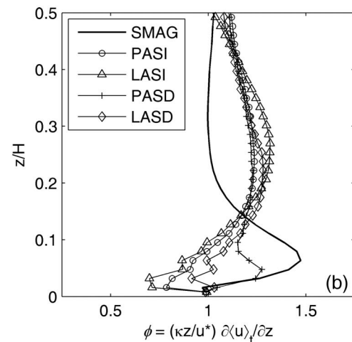
FIG. 2. (a) Normalized streamwise mean velocity profiles; the solid black line is the log law profile with z_0/H = 10^{-4} , (b) nondimensional mean velocity gradients for different SGS models.
