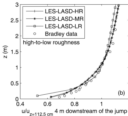
FIG. 16. Evolution of velocity profiles after an abrupt change in surface roughness: sensitivity to grid resolution for the LASD SGS model. HR is for high resolution ( 160 \times 64 \times 200 ), MR is for medium resolution ( 120 \times 48 \times 150 ), and LR is for low resolution ( 80 \times 32 \times 100 ).
