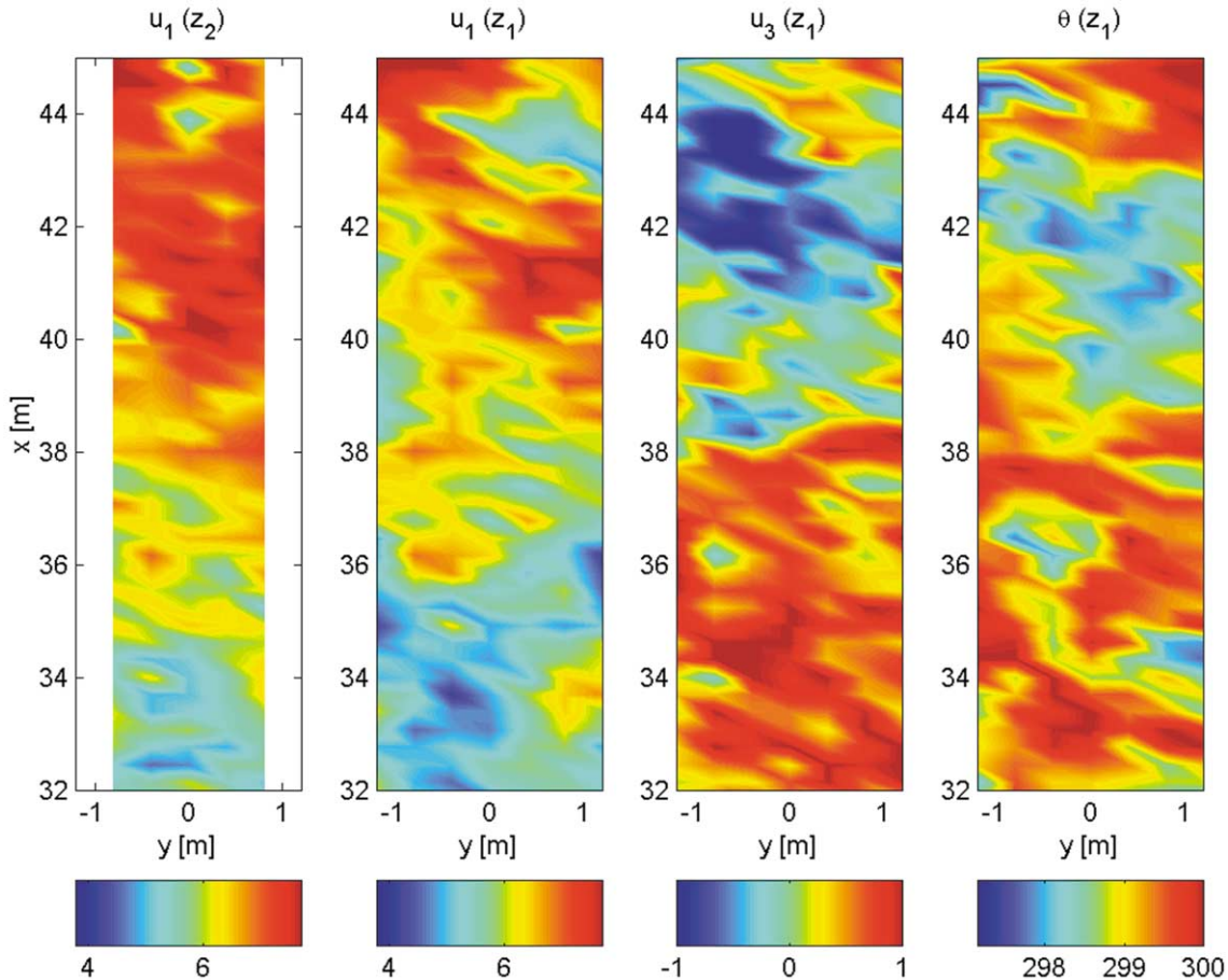
Fig. 3. Horizontal contour plots of the streamwise velocity ( u_1 in \text{m s}^{-1} ) at the two heights ( z_1 and z_2 ), vertical velocity ( u_3 in \text{m s}^{-1} ) at z = z_1 , and temperature ( \theta in K) also at z = z_1 , corresponding to measurement period D (unstable).
