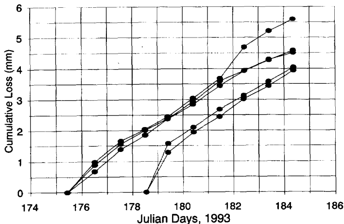
Fig. 2. Cumulative water loss (in mm) from microlysimeters in the sand-dominated portion of the Owens Lake playa.
