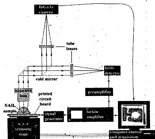
FIG. 1. NAIL Confocal scanning thermal emission microscope configuration.
