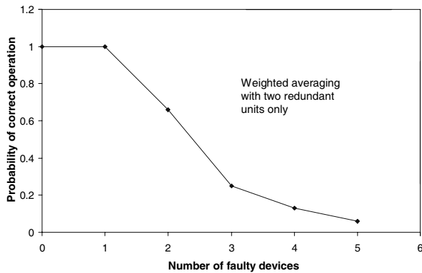
Fig. 8: Probability of correct operation with two redundant units.
