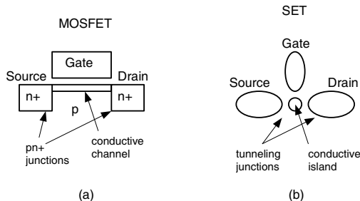
Fig. 1: Simplified structure of a MOSFET (a), compared with that of an SET (b).
