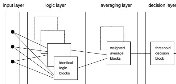
Fig. 2: The proposed fault-tolerant architecture based on multiple layers.
