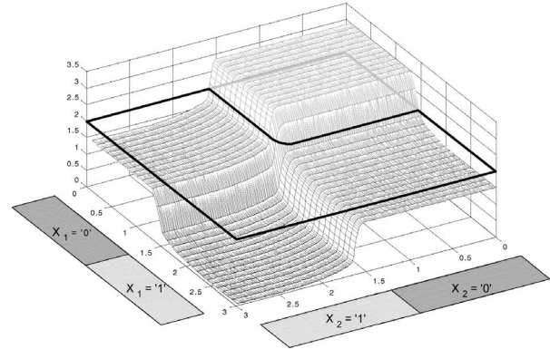
Fig. 5: Output transfer function generated by the averaging layer of the two-input NOR circuit, with a total of four device failures in both of the second-layer logic blocks. It is seen that the correct output can still be obtained with the proper threshold decision in the fourth layer.
