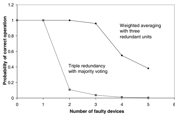
Fig. 9: Probability of correct operation with three redundant units.
