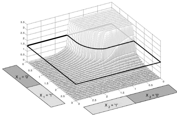
Fig. 4: Output transfer function generated by the averaging layer of the two-input NOR circuit, showing correct operation (no device failures). The fourth-layer decision threshold is also indicated.
