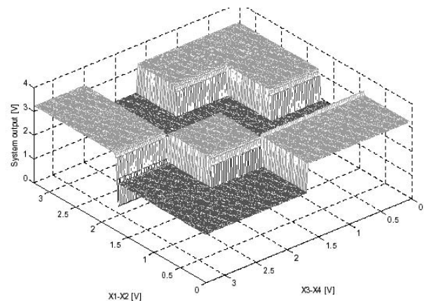
Fig. 6: Transfer function surface of a 4-input mapping onto a 1-output, with a large number of distributed errors.
