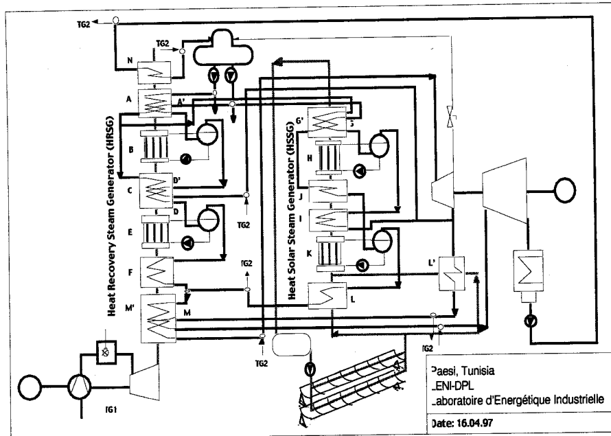
Fig 4 : Flowsheet of the alternative of an ISCCS with the highest efficiency and dual pressure steam generators
