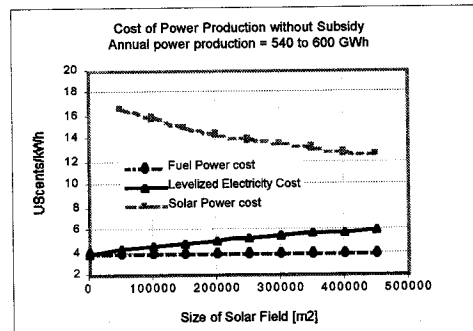
Fig. 7 : Power costs versus size of
