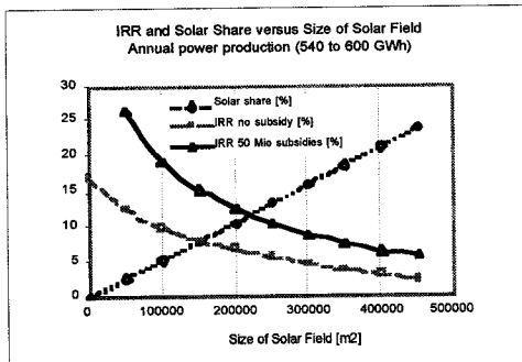
Fig. 6 : IRR and solar share versus size
