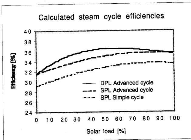
Fig.5 : Calculated steam cycle efficiencies
