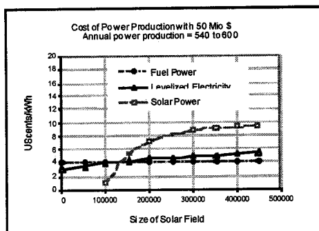
Fig.8 : Power costs versus size of solar field (with subsidy)
