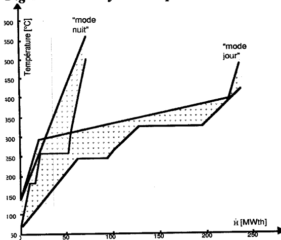
Fig 2 : Optimized composites for two extreme operation modes: CC-night and ISCCS-day
