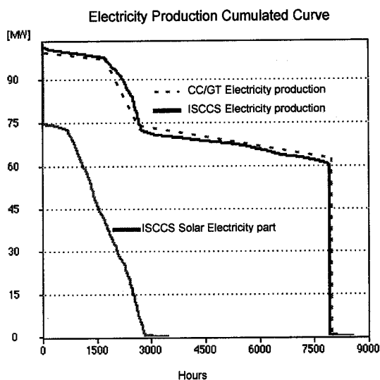
Fig.9: Cumulated curve of the Electricity production
