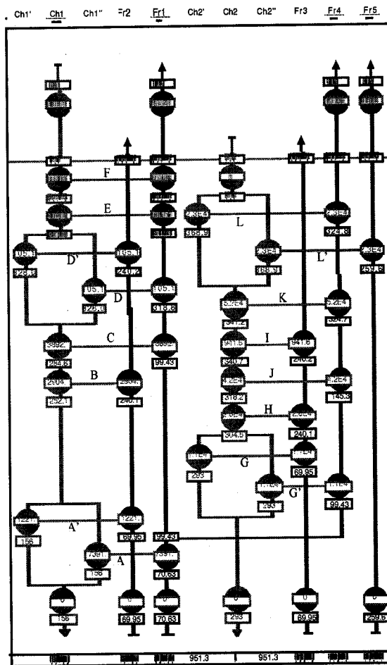
Fig 3 : Heat exchanger networks
