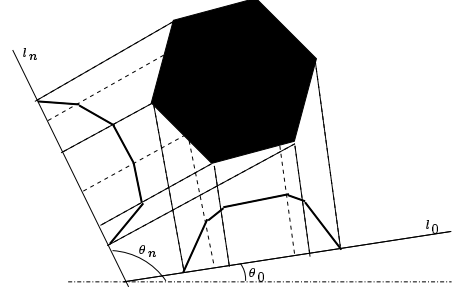
Figure 2: Bilevel Polygon The projection of a bilevel polygon onto an arbitrary line is a piecewise linear signal. For the signal with M vertices, 2M sample values of the filtered Radon transform taken along each of the M + 1 different directions uniquely specify the signal.
