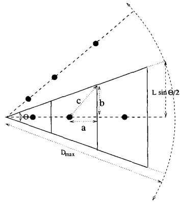
Figure 8: Deriving the R_{max} constraint in 2d placement. For any of the Voronoi cells, the furthest points are the corners of the cell.
