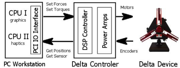
Figure 4 – control system overview
