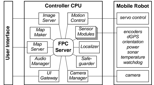
Figure 2. Controller architecture
