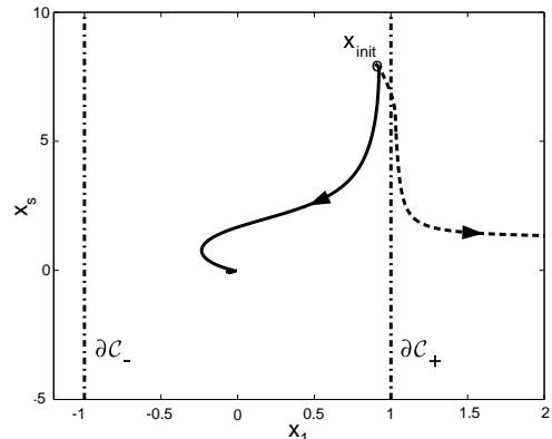
Figure 1: Non-zero initial conditions ( x_{init} ); dashed: reference controller, solid: continuous nonlinear controller.
