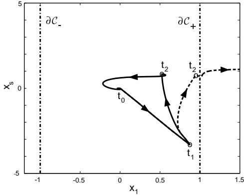
Figure 2: Large disturbance; dashed: reference controller, solid: continuous nonlinear controller.
