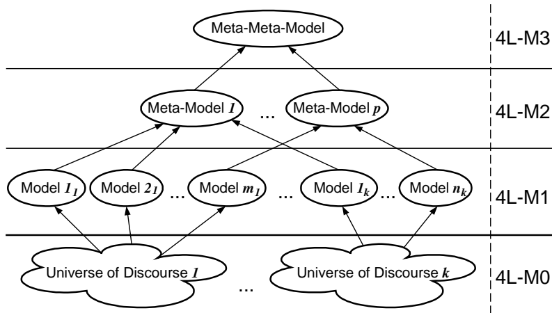
Figure 1: Four-level ontological approach (indexes k , m , n and p are natural numbers).
