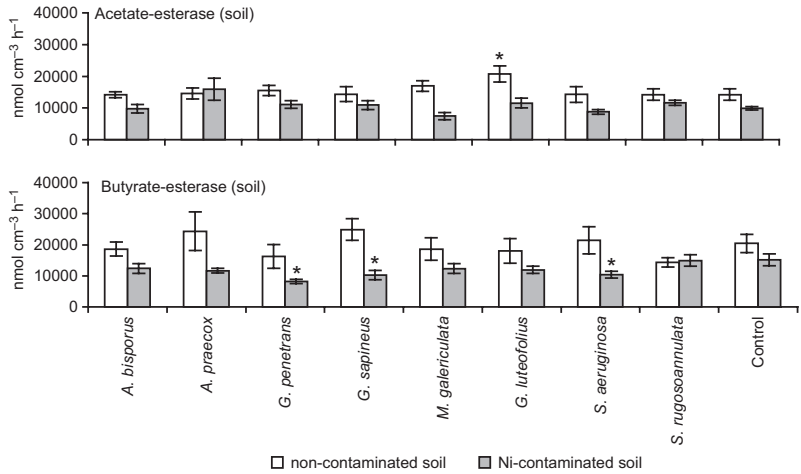
Fig. 4. Acetate-esterase and butyrate-esterase activities in the organic layer of Ni-contaminated (20 mg [kg soil] -1 ) and non-contaminated soil ( n = 6 ). Bars are standard errors of the mean. Statistical differences ( t -test: p < 0.05 ) between fungus-inoculated and non inoculated control soil are indicated with asterisks (*).
