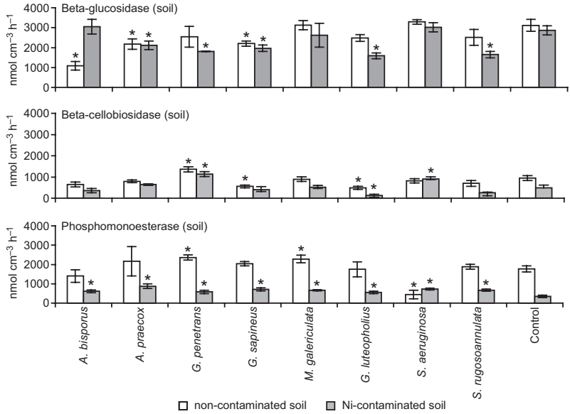
Fig. 3. \beta -Glucosidase, \beta -cellobiosidase and phosphomonoesterase activities in the organic layer of Ni-contaminated (20 mg [kg soil] -1 ) and non-contaminated soil ( n = 6 ). Bars are standard errors of the mean. Statistical differences ( t -test: p < 0.05 ) between fungus-inoculated and non inoculated control soil are indicated with asterisks (*).
