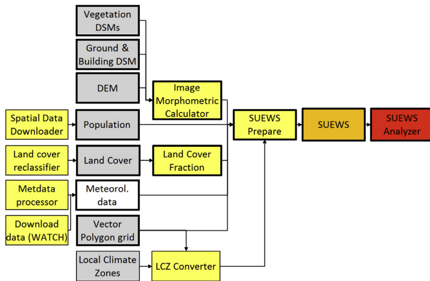
Fig. 3. Workflow and geodata for analysing urban energy balance using the SUEWS model. Bold outlined boxes are mandatory items. In some cases alternatives are shown. Yellow, orange and red indicates pre-processor, processor and post-processor tools, respectively (consistent with Fig. 1). Grey boxes indicate geodatasets and white boxes other types of data. DEM – digital elevation model, DSM – digital surface model, LCZ – local climate zones. It is strongly recommended that all geodata used are transformed into the same projected coordinate system. Model areas need to be defined in a vector polygon layer. For the meteorological forcing, users could manipulate their own data ( Metadata Processor ), use the WATCH – WFDEI climatological data set ( Download data (WATCH) ) or link to their own already-prepared data. (For interpretation of the references to colour in this figure legend, the reader is referred to the web version of this article.)
