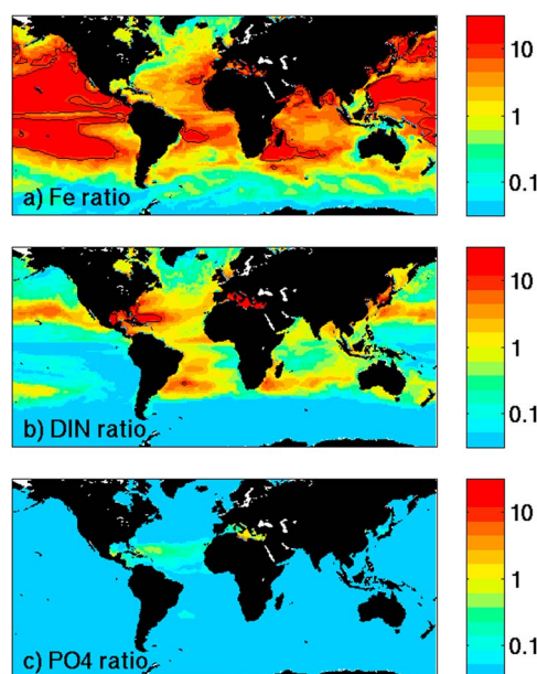
Figure 4. Relative contribution (%) of dust to the model-derived supply of nutrients to the top 100 m on the ocean for (a) Fe, (b) dissolved inorganic nitrogen (DIN), and (c) PO 4 . The “in water” supplies include vertical and horizontal advection and diffusion, as well as remineralization of organic matter. Contour is 10%. Color bars are in log scale.
