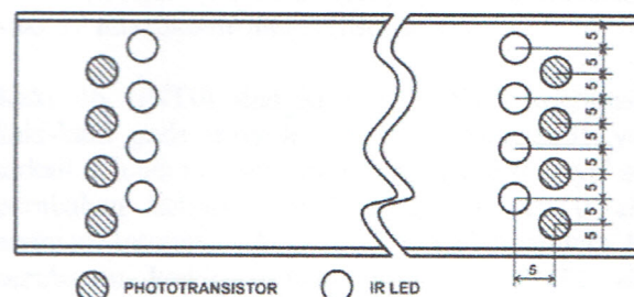
Gambar 2 Susunan IR LED-Phototransistor
