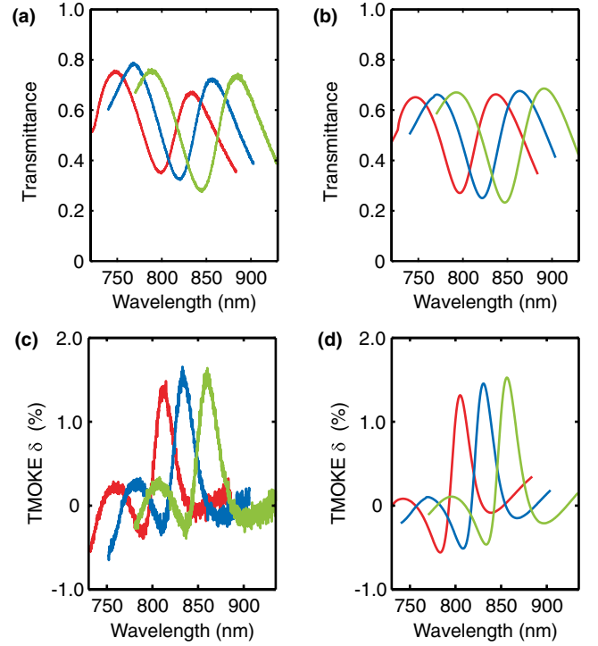
FIG. 3. (a) Measured and (b) simulated transmittance for the structures of a 450-nm period (red lines), a 475-nm period (blue lines), and a 500-nm period (green line). (c) Measured and (d) simulated TMOKE for the structures of a 450-nm period (red lines), a 475-nm period (blue lines), and a 500-nm period (green lines). Illumination is TM polarized with a 9^\circ incident angle. An external magnetic field of 160 mT is applied.
