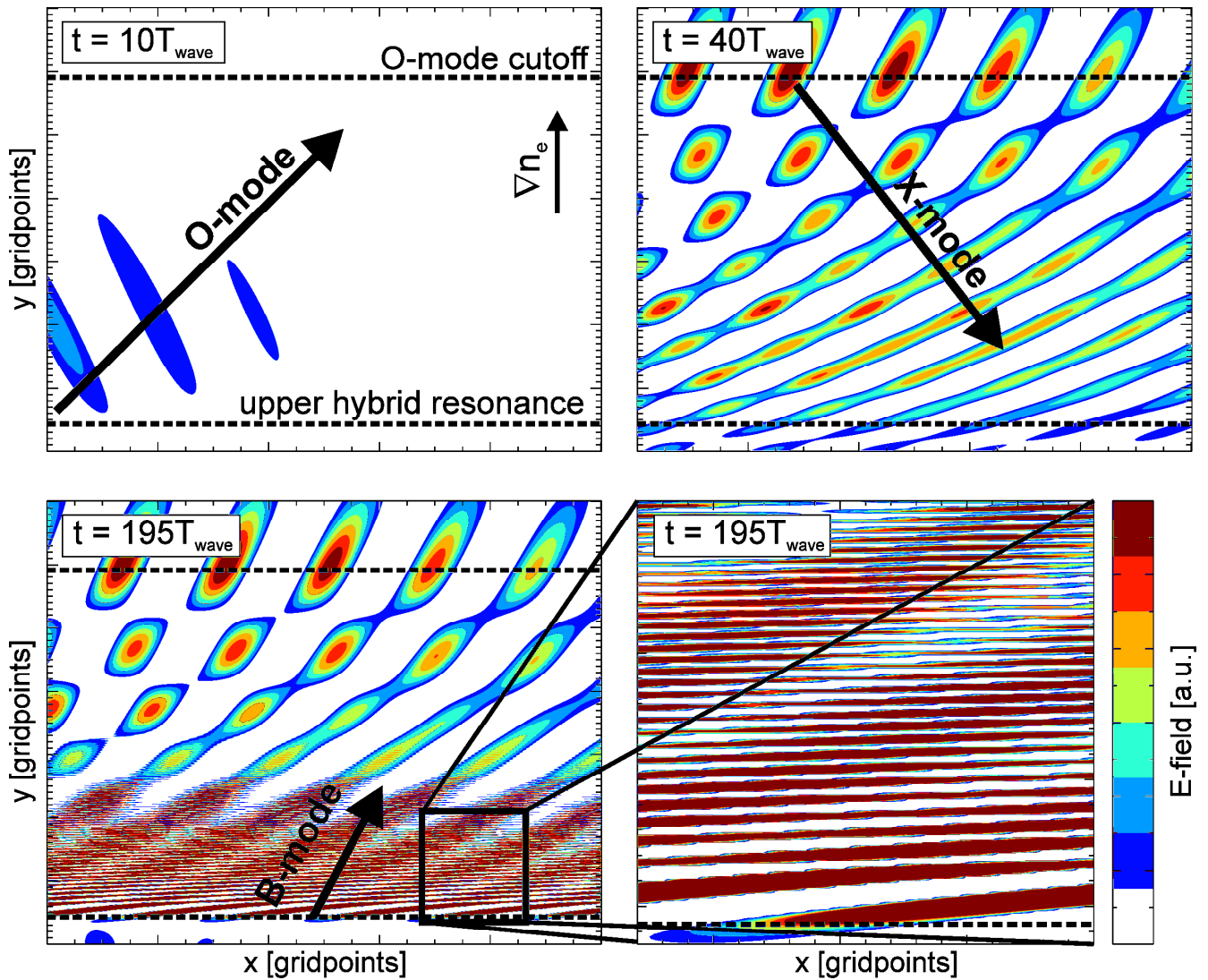
Fig. 1. O-X-B mode conversion. Plotted are the positive values of the wave electric field. \mathbf{B}_0 is parallel to the x-axis, \nabla n_e is parallel to the y-axis. The wave is incident from the lower left side. Coloured plot in online version.
